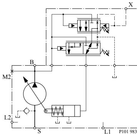
LB Schematic
