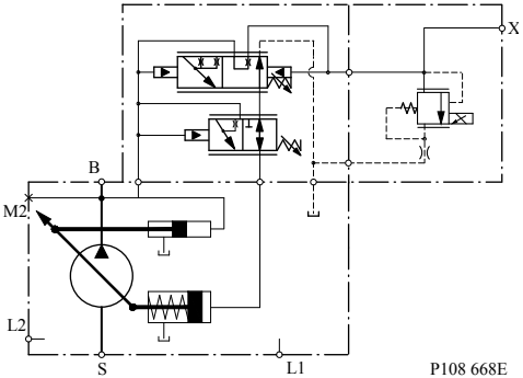
Schematic
